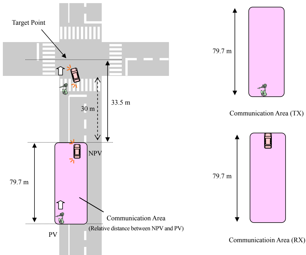
Fig. C.3-1: Communication area for left-turn collision prevention system
