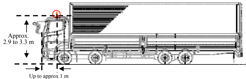
Appendix Fig. C.2-2: Large vehicle: 1 m behind the front of the vehicle, on the cabin roof
