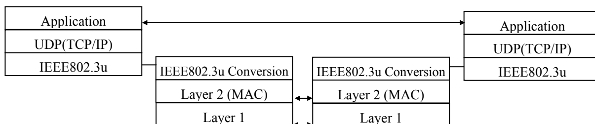
Appendix Fig. B.1-1: Example of Additional Specification of Inter-application Communication (IP Packet Transparent Communication)
